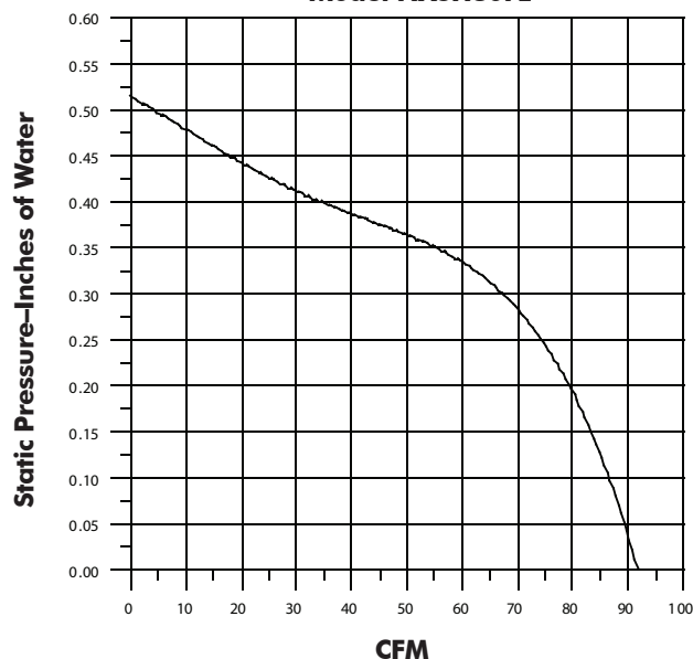
NuVent Product Performance Model NXSH80FL
